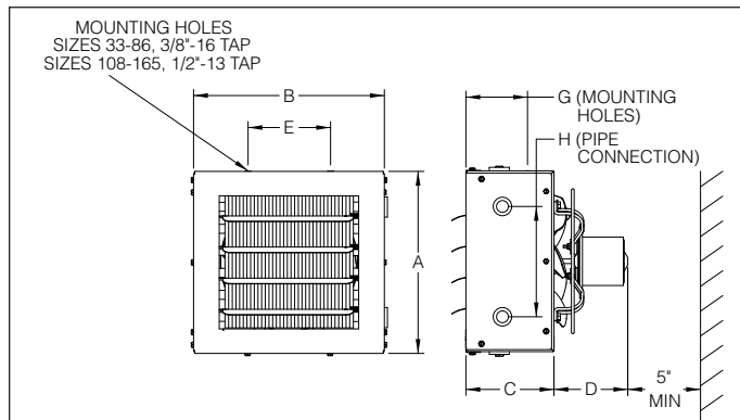
Figure 12.3 - Model Dimensions WSC 18-165
