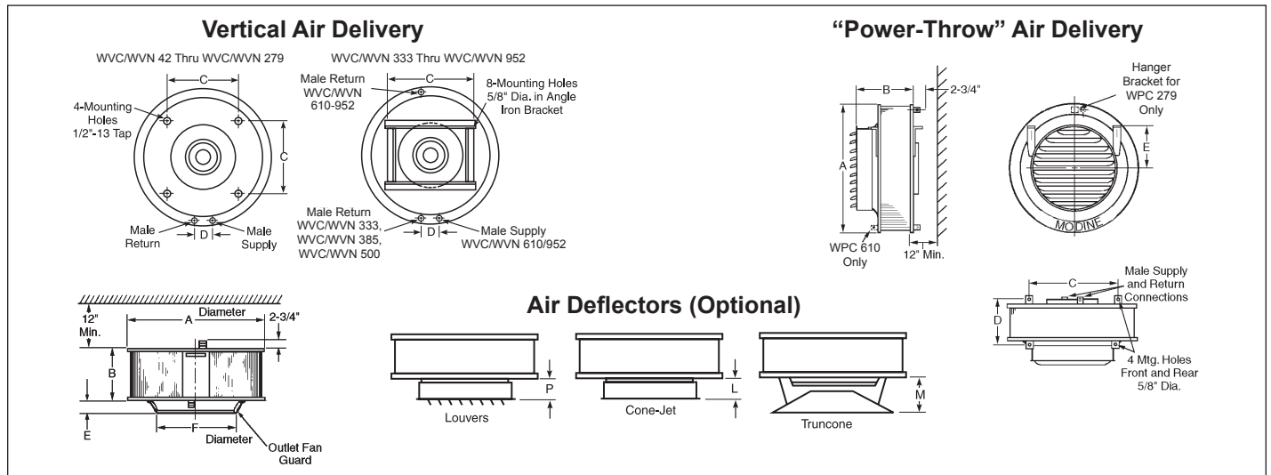
Figure 13.1 - Model Dimensions WVC/WVN and WPC/WPN
