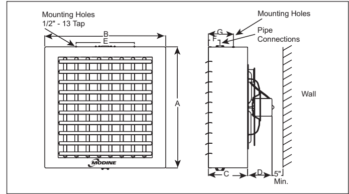
Figure 12.4 - Model Dimensions WSC 193-340 ①
