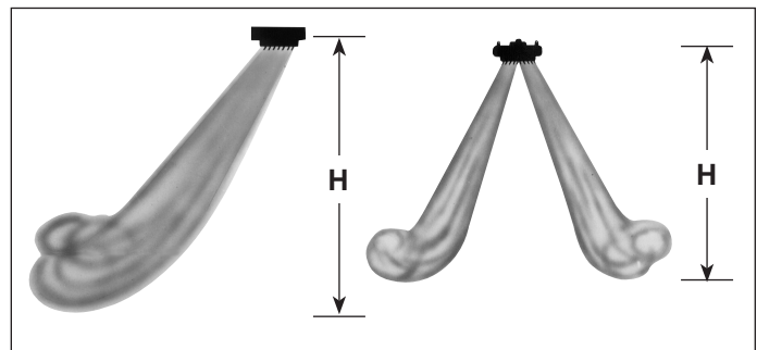
Figure 4.6 - Vertical Truncone
